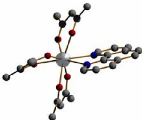
\text{Tb}(\text{acac})_3\text{Phen}
